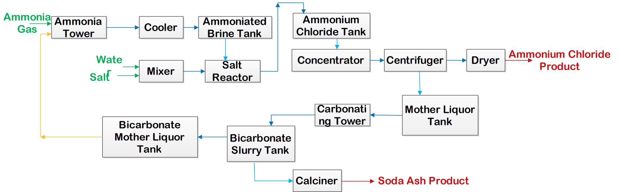
Figure: Manufacturing of Ammonium Chloride by dual salt process
